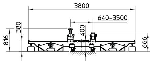
DIMENSION OVERVIEW
